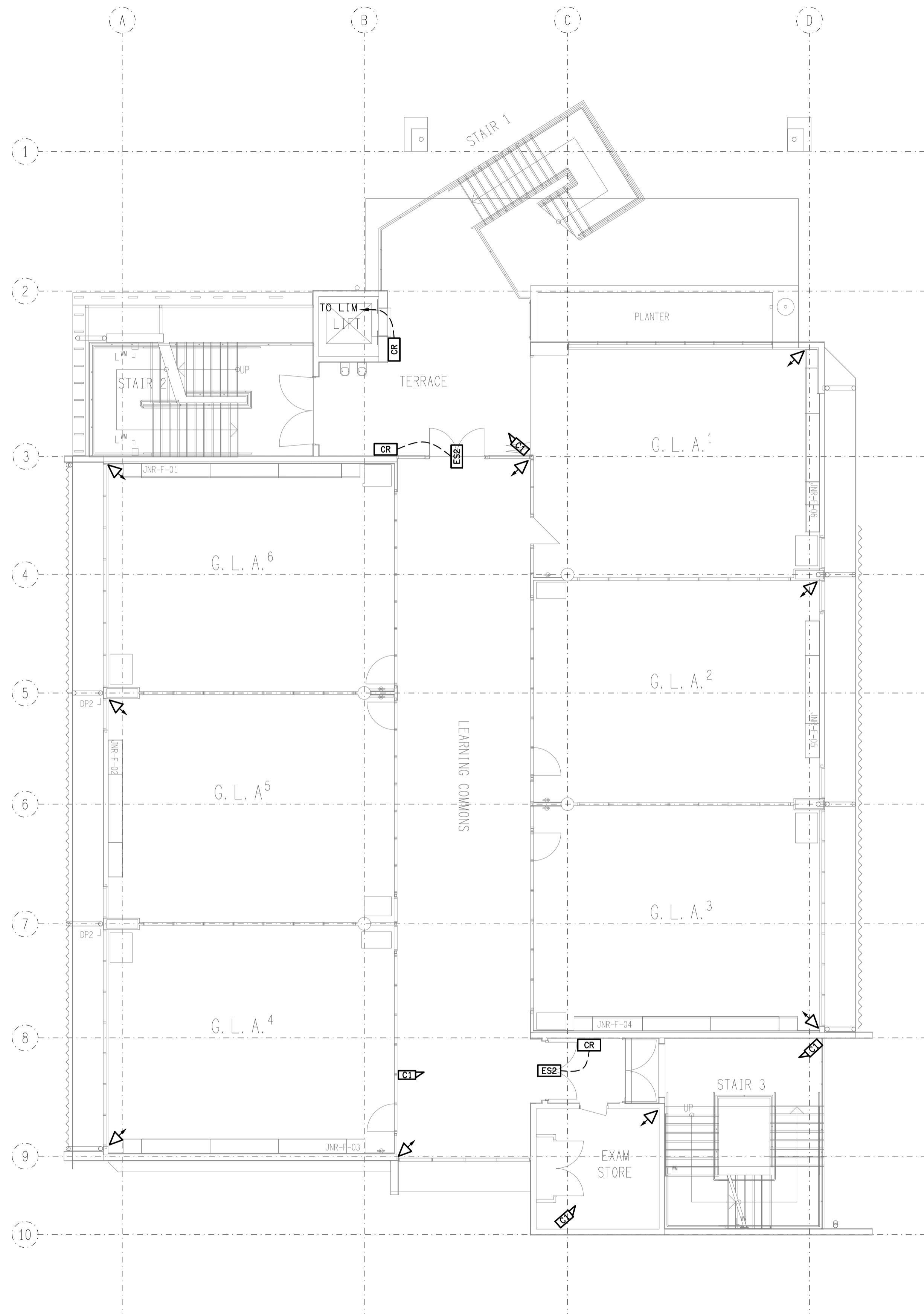
LEVEL 1 SECURITY PLAN SCALE 1:100
